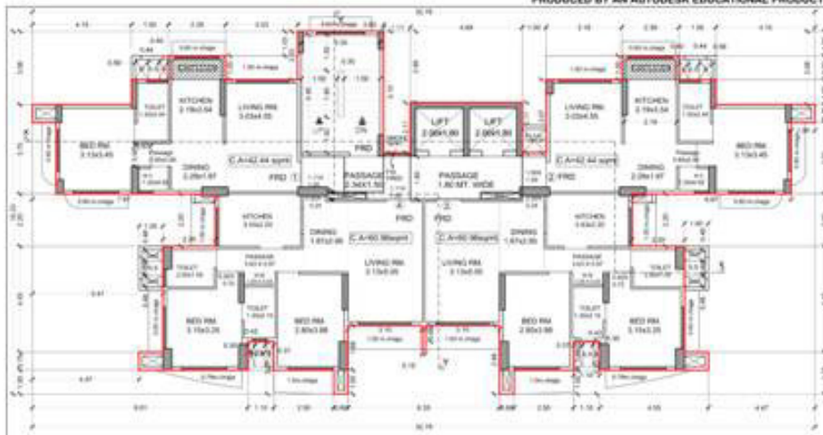
TYPICAL FLOOR PLAN (4th TO 7th, 9th to 14th) SCALE: 1/32"
