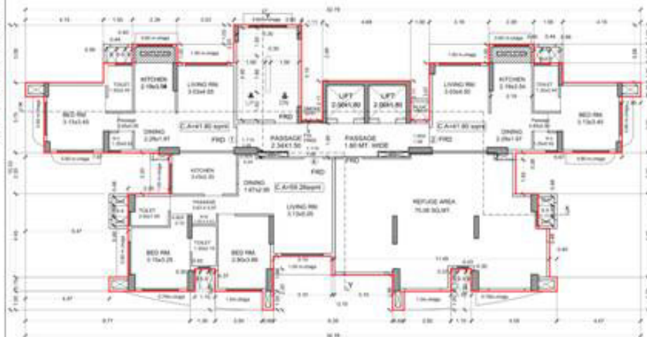
8TH FLOOR PLAN (REFUGE) SCALE: 1/32"
