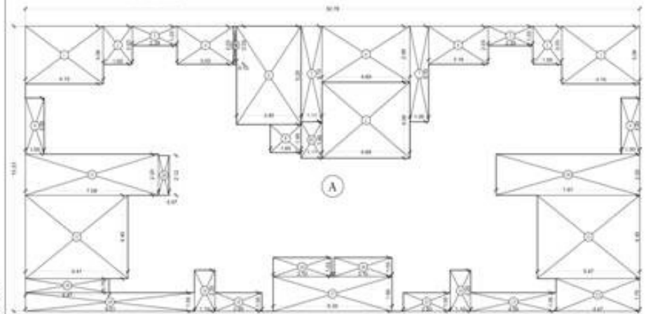
TYP AREA DIAGRAM (4th TO 7th, 9th to 14th, 17th & 18th) SCALE: 1/32"
