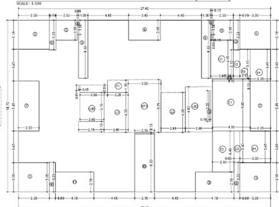
LINE AREA DIAGRAM OF GROUND FLOOR PLAN (TOWER-G) SCALE: 1:100
