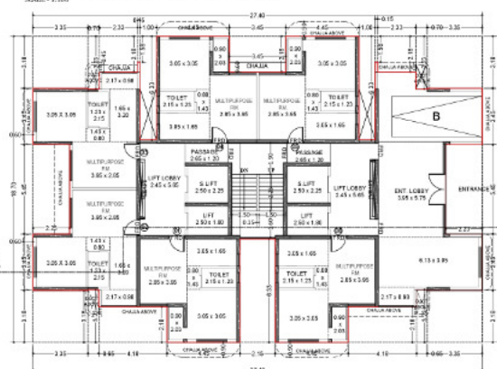
GROUND FLOOR PLAN (TOWER-G) SCALE: 1:100
