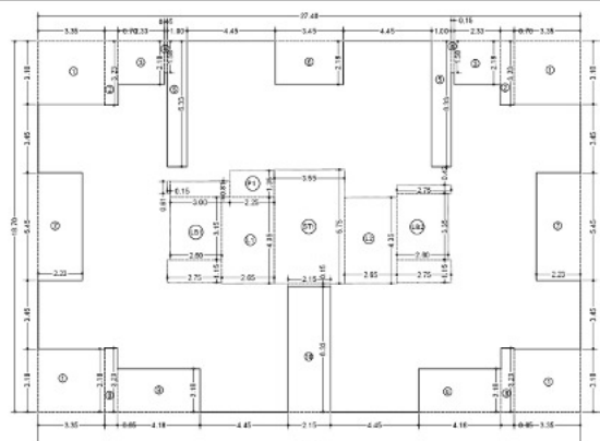
LINE AREA DIAGRAM OF 1ST TO 4TH TYPICAL FLOOR PLAN (TOWER-G) SCALE: 1:100
