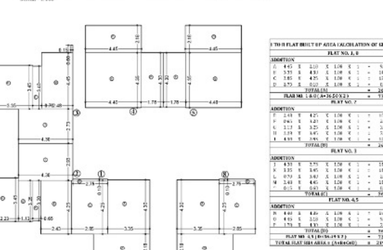
I TO R PLAT AREA DIAGRAM OF GROUND FLR (TOWER-G) SCALE: 1:100
