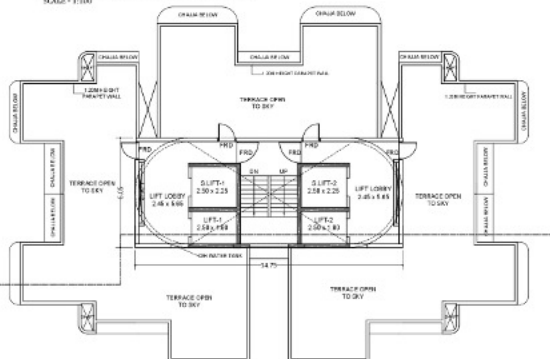
TERRACE FLOOR PLAN (TOWER-G) SCALE: 1:100
