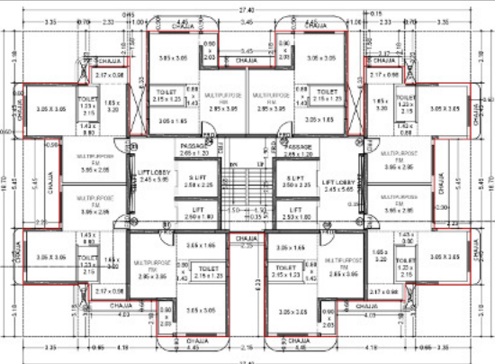
1ST TO 4TH TYPICAL FLOOR PLAN (TOWER-G) SCALE: 1:100
