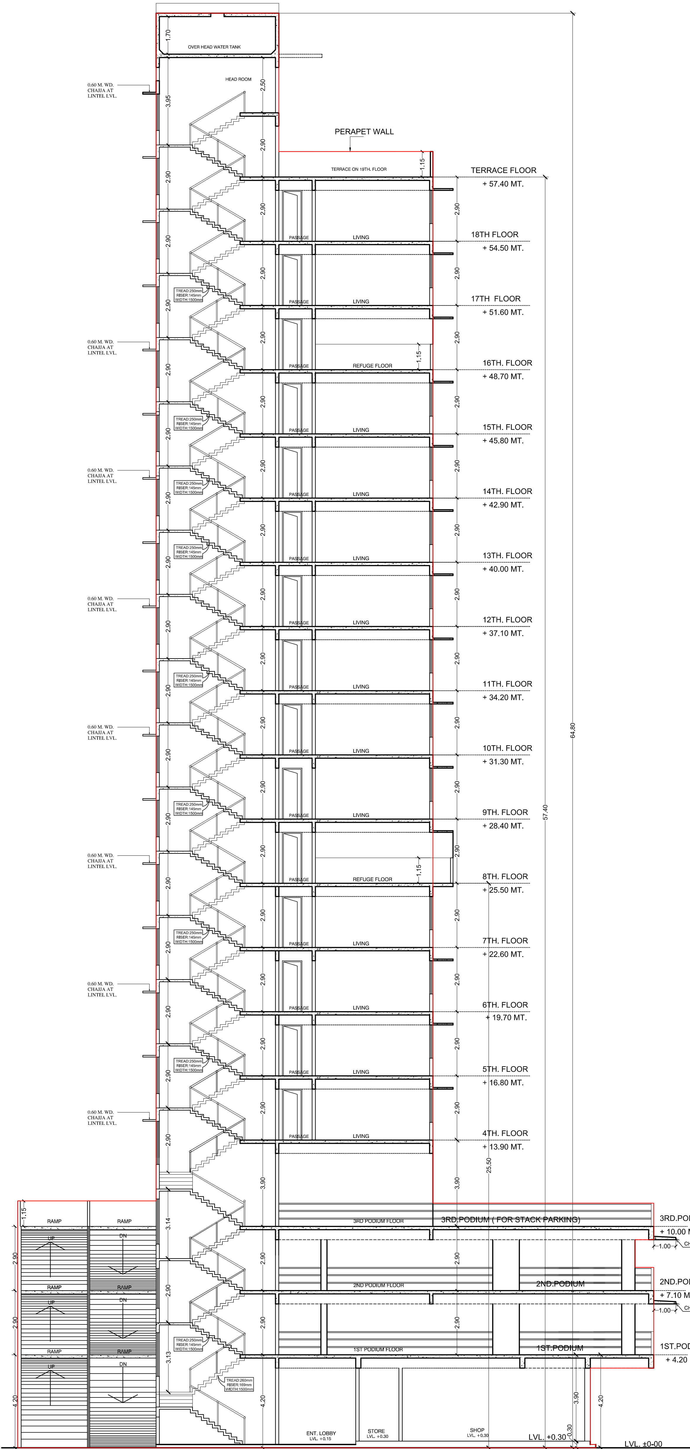
SECTION AT Y-Y SCALE 1:100
