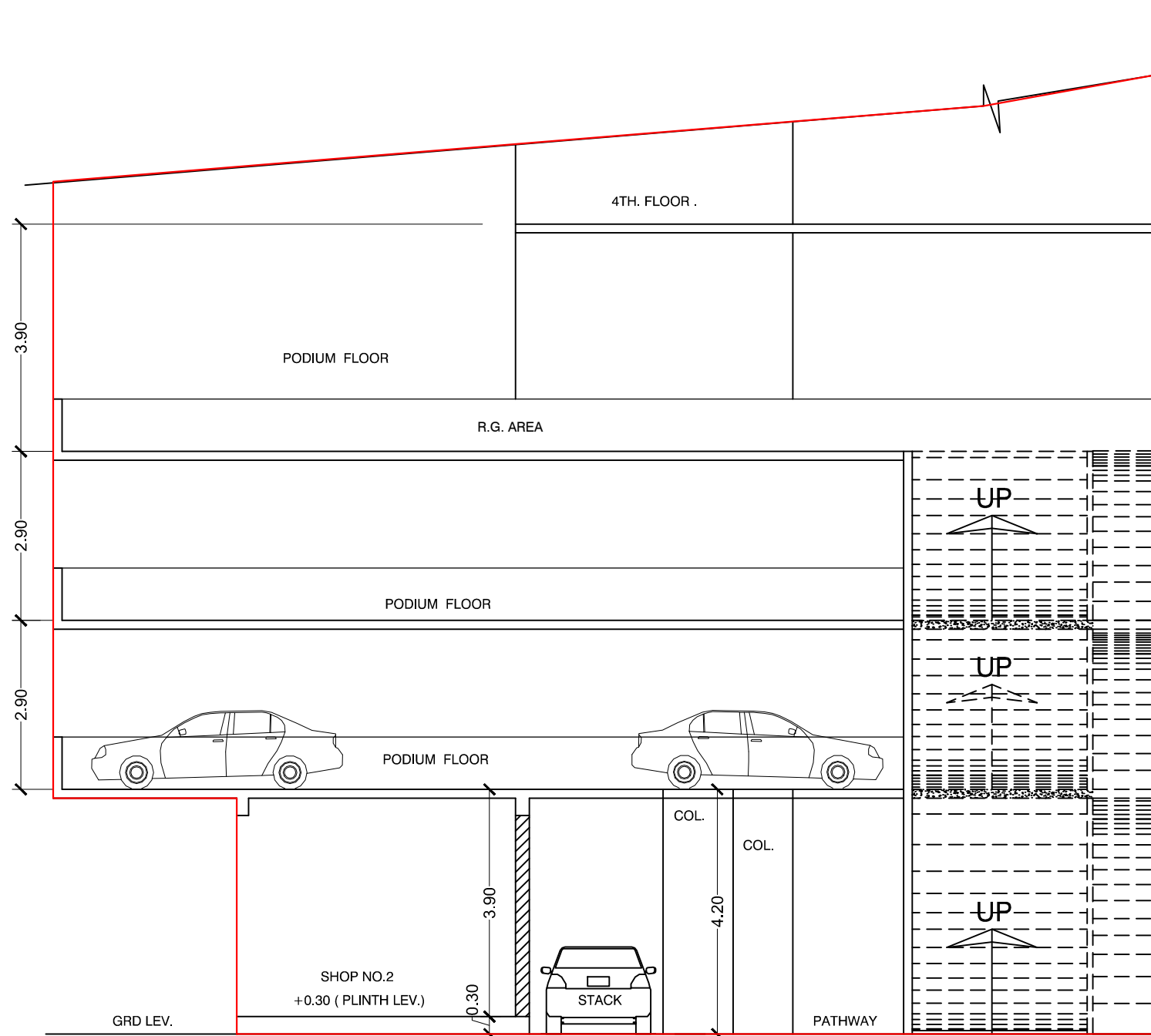
SECTION AT P-P SCALE 1:100
