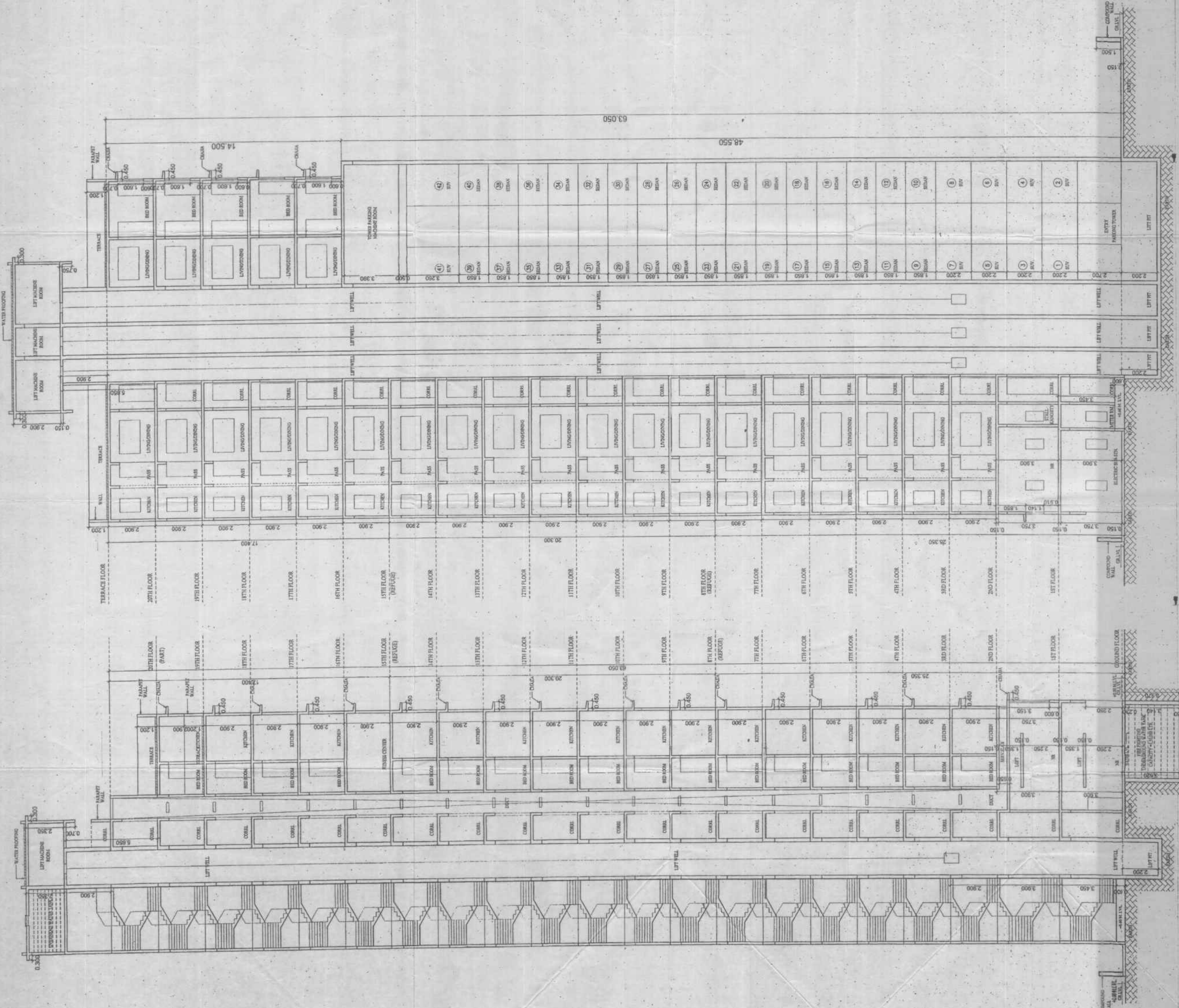
SECTION B-B SCALE 1:100
